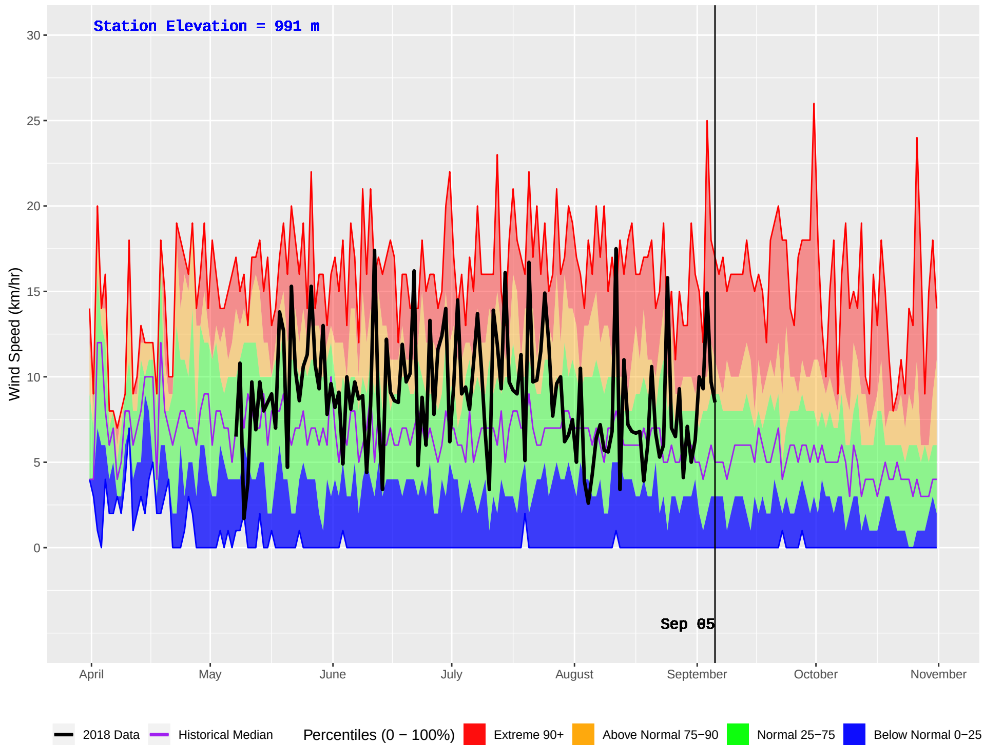
TROUT LAKE (387) : Historical (1987–2016) and Current (2018) Daily Wind Speed
