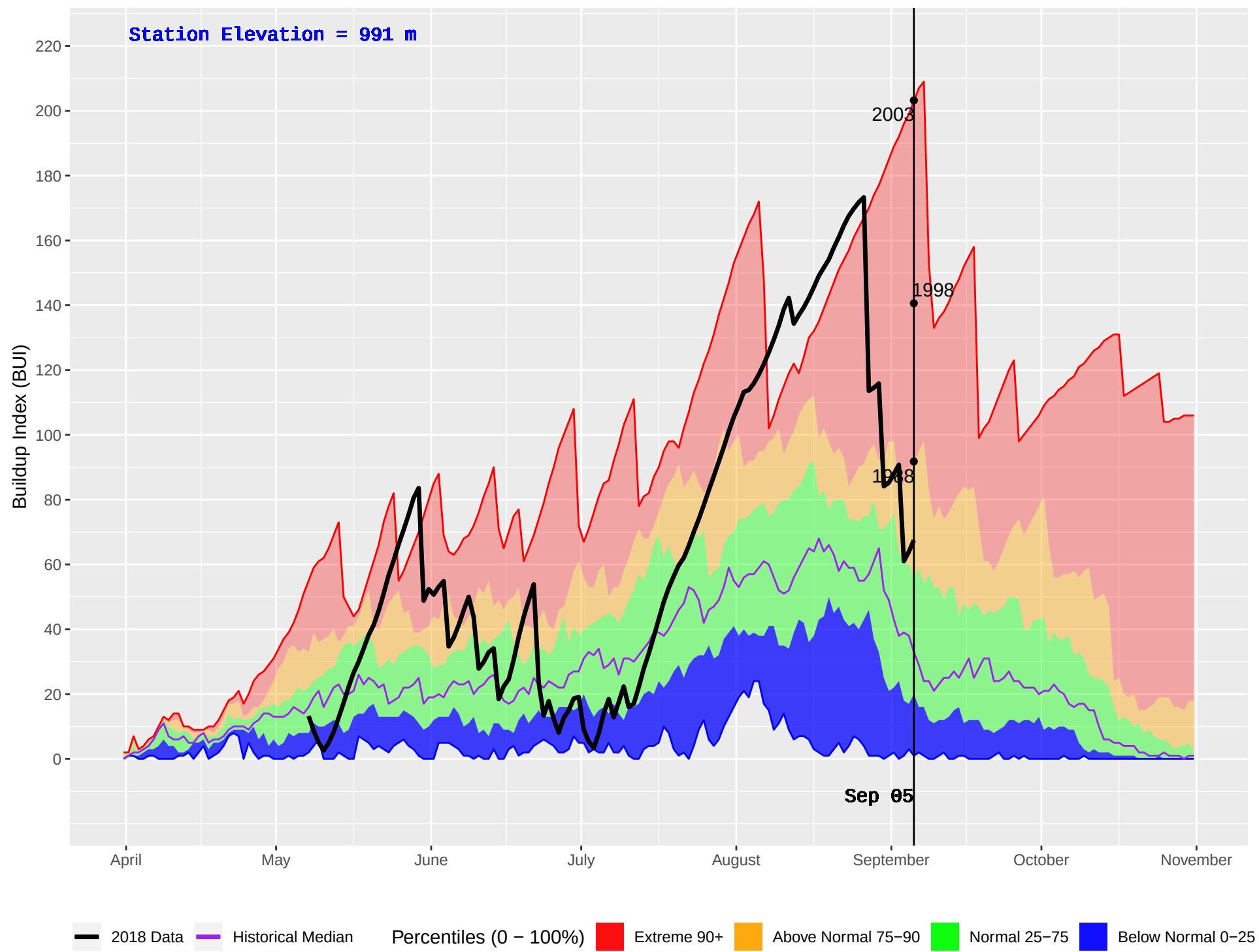
TROUT LAKE (387) : Historical (1987–2016) and Current (2018) Daily Buildup Index (BUI)
