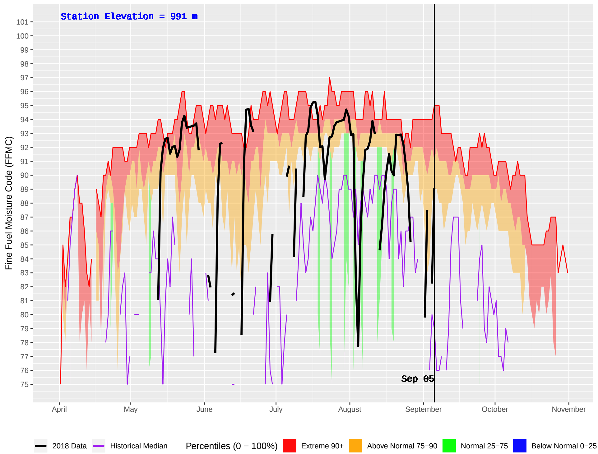
TROUT LAKE (387) : Historical (1987–2016) and Current (2018) Daily Fine Fuel Moisture Code (FFMC)
