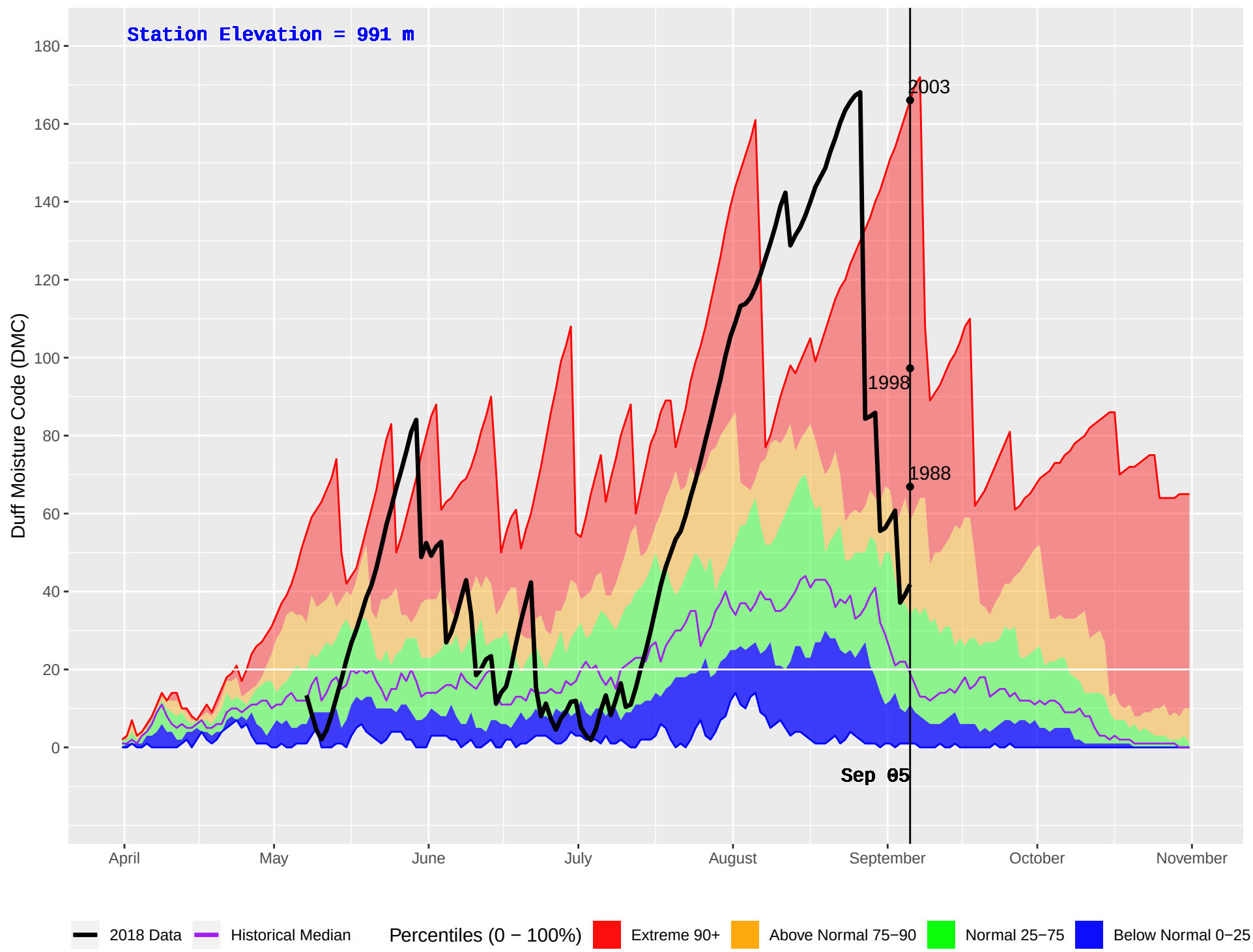
TROUT LAKE (387) : Historical (1987–2016) and Current (2018) Daily Duff Moisture Code (DMC)
