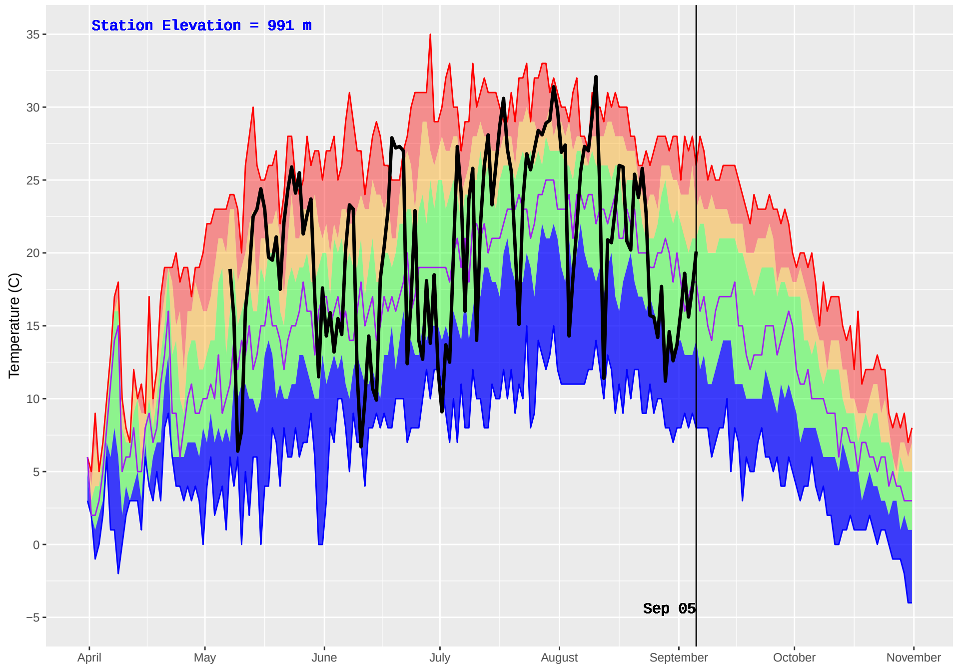
TROUT LAKE (387) : Historical (1987–2016) and Current (2018) Daily Temperature
